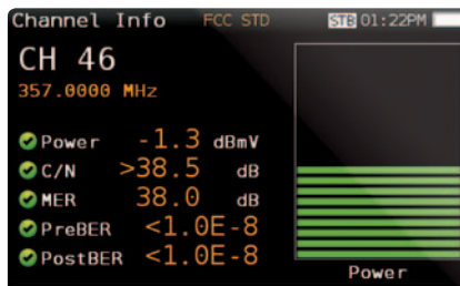
CHANNEL INFO All in a quick glance
