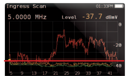
REVERSE PATH INGRESS SCAN Maximum, average, peak
