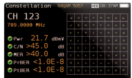
CONSTELLATION DISPLAY Fine-tune your digitals
