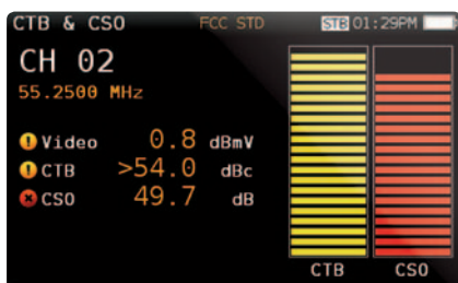
CSO & CTB Deep dive into those analogs
